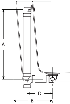
DRAIN/OVERFLOW
